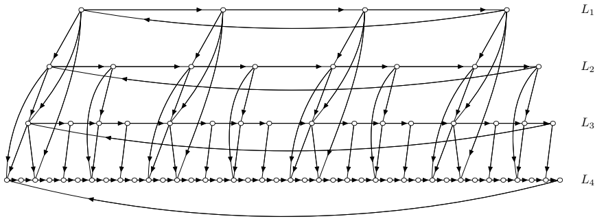
Figure 2.4. Layers L_1 to L_4 of the (f, 4) -layered wheel when f(4) = 3
